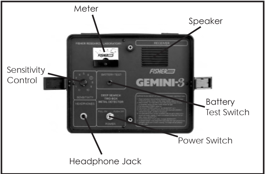
Figure 3. Receiver
